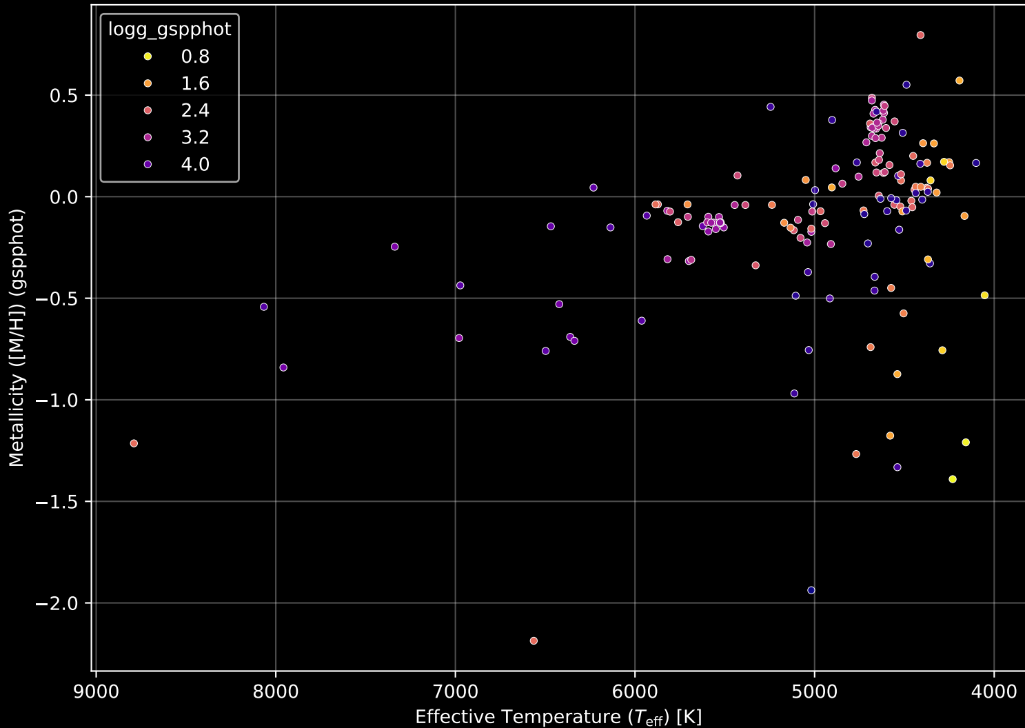
APOGEE DR17 Field: [N362] Stellar Population Parameters (n= 160)
