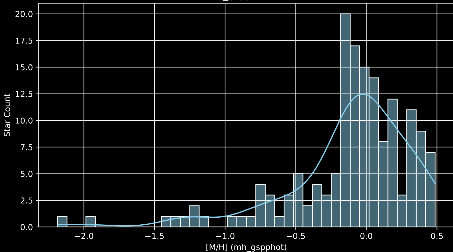
APOGEE DR17 Field: [N362 [M/H] (mh_gspphot) (n= 157)
