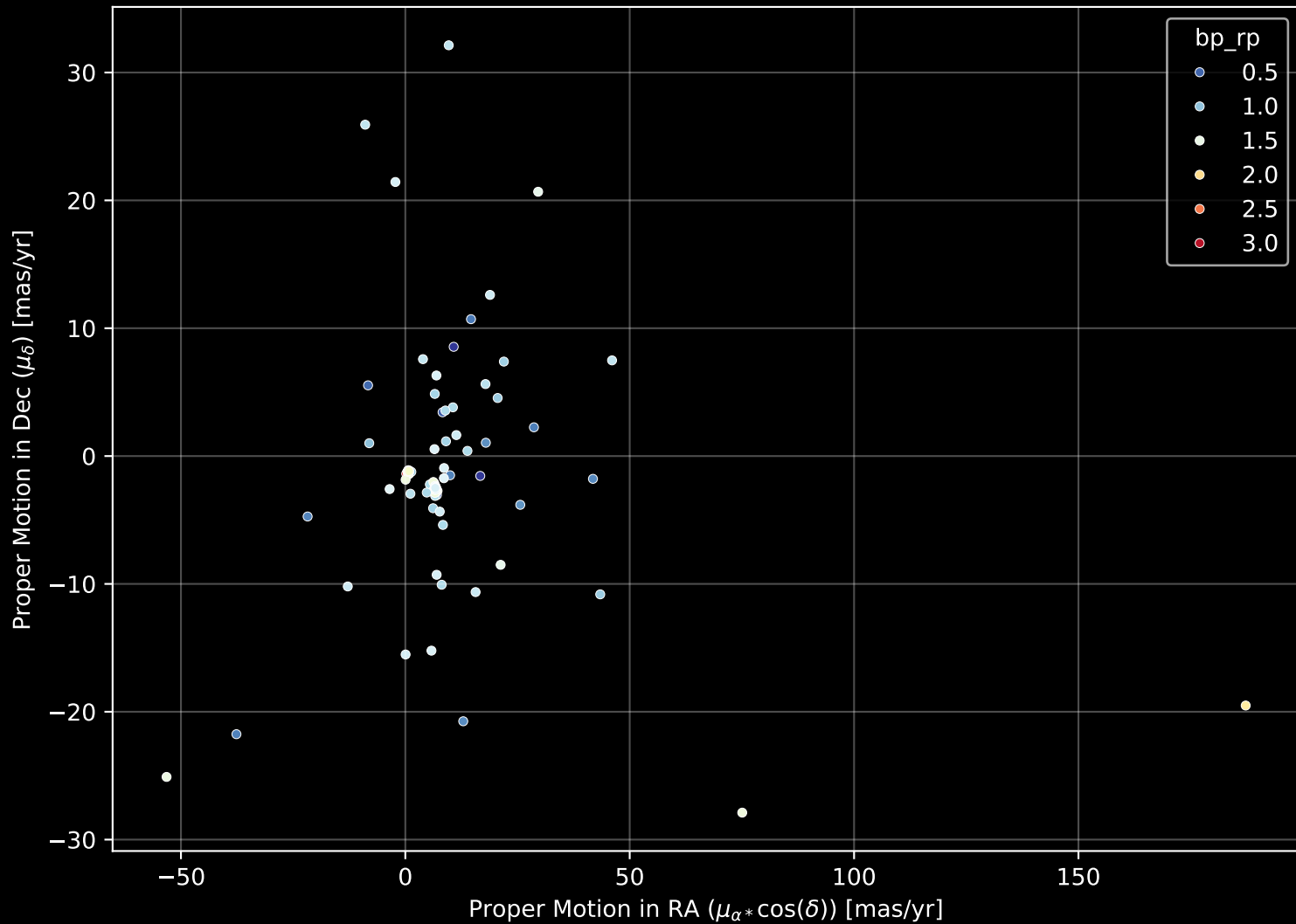
APOGEE DR17 Field: [N362] Proper Motion Diagram (n= 160)
