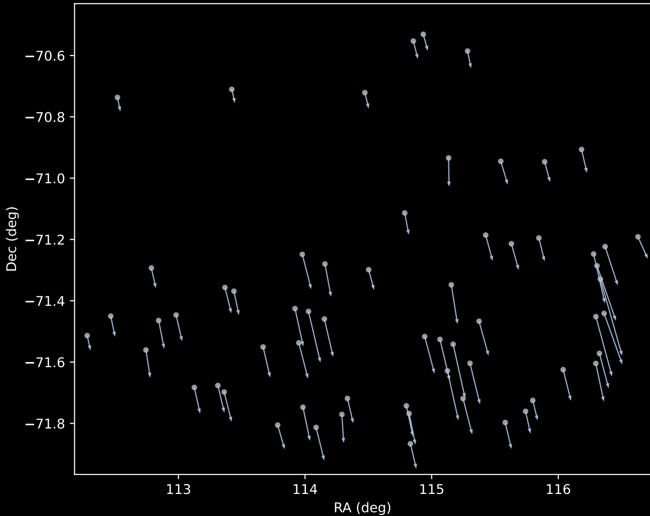
APOGEE DR17 Cluster 1 Proper Motion Vectors (n=62)
