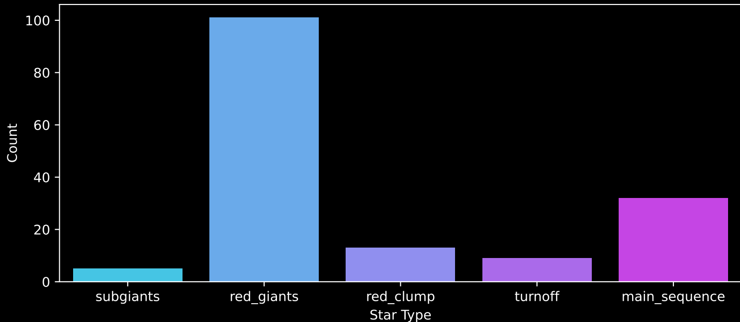
APOGEE DR17 Field: [N362] Count plot of Star Type
