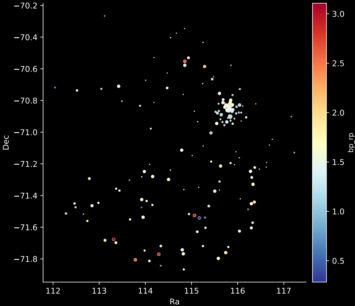
APOGEE DR17 Field: [N362] Stars: 160
