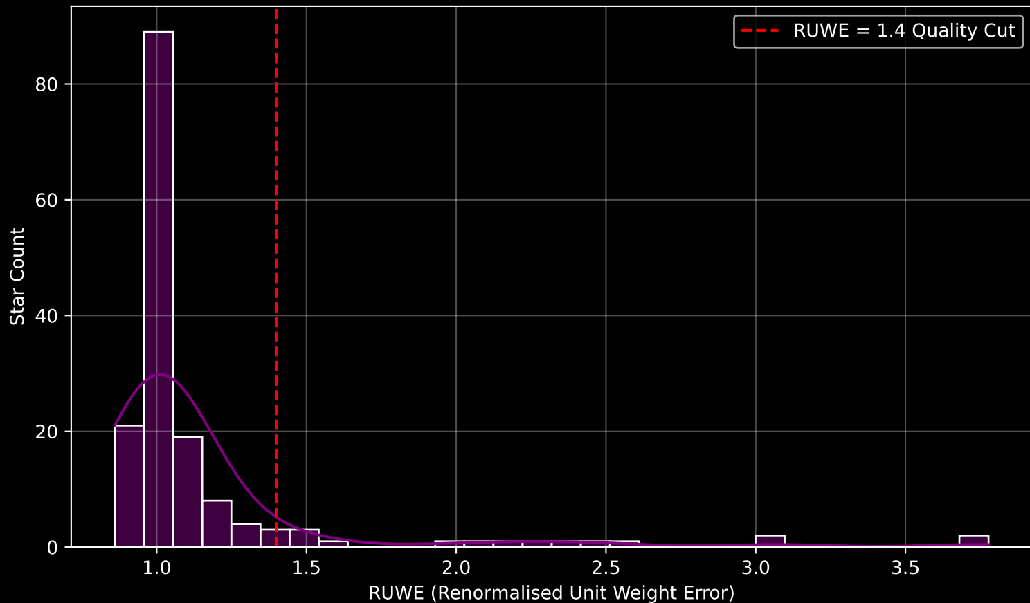
GAPOGEE DR17 Field [N362] RUWE Distribution (n= 159)
