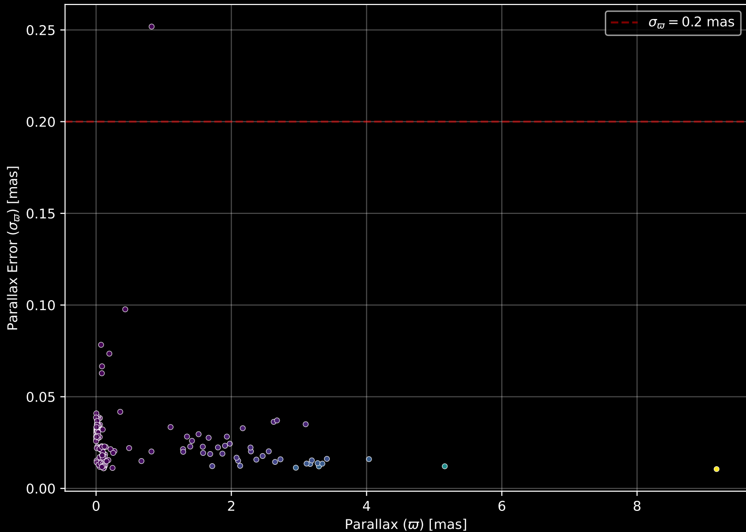
APOGEE DR17 Field: [N362] Parallax Quality (n= 160)
