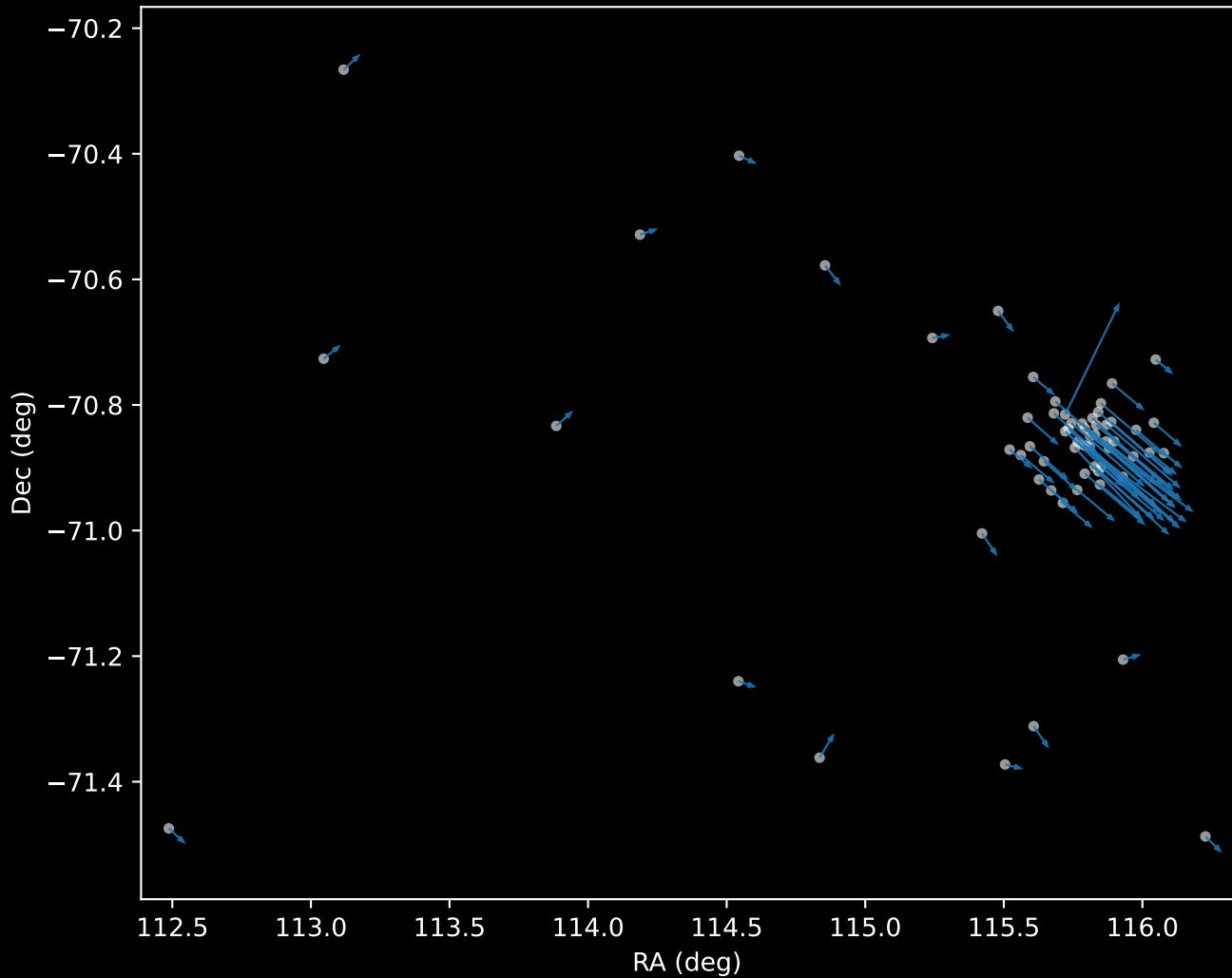
APOGEE DR17 Cluster 0 Proper Motion Vectors (n=63)
